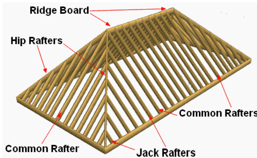
Figure 1. Example of Hip Roof structure
